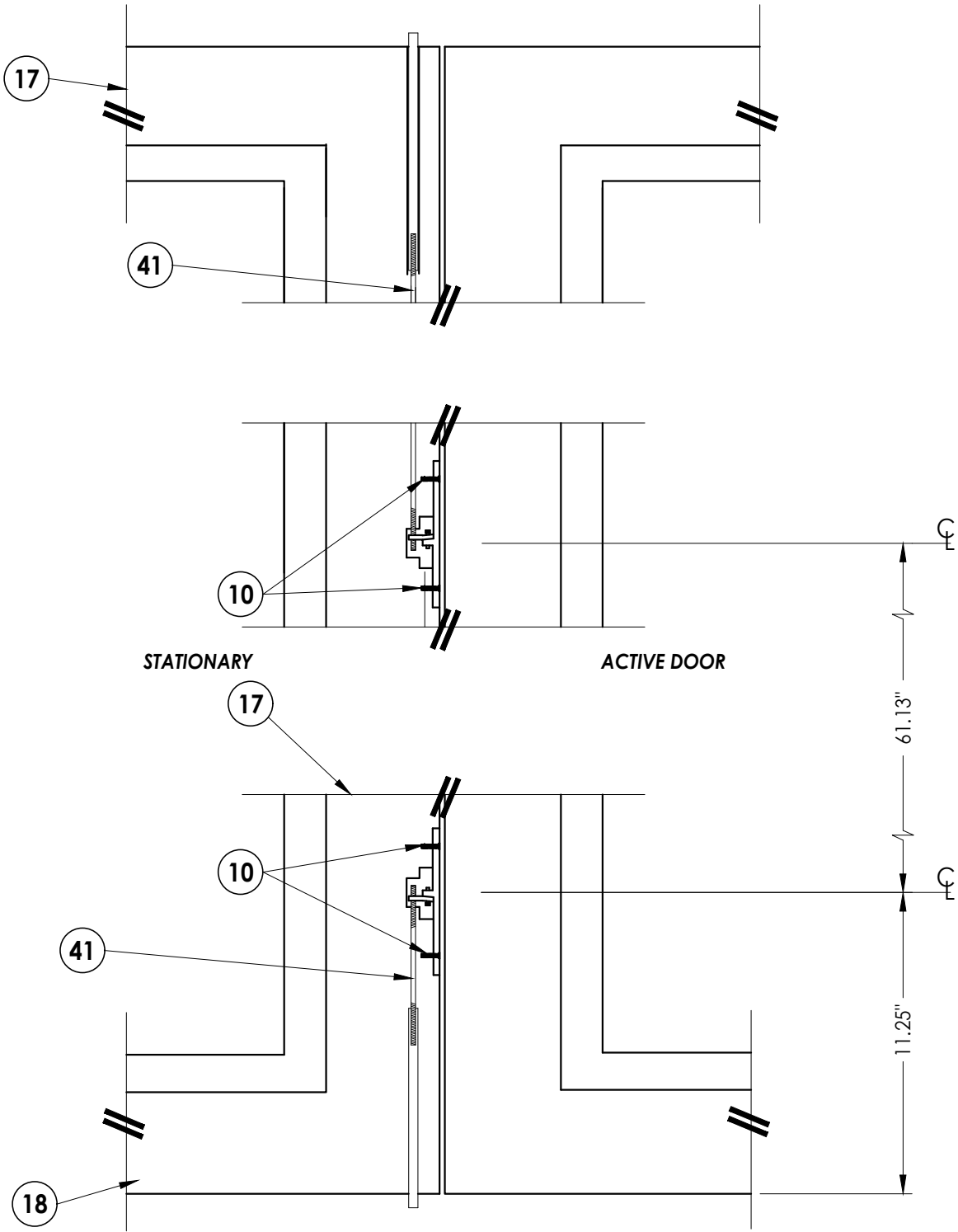
FLUSH BOLT DETAIL
