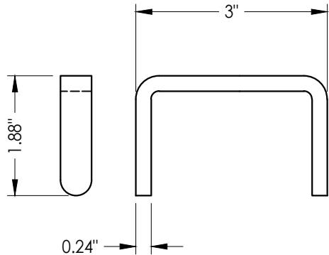
34 LATCH KEEPER
