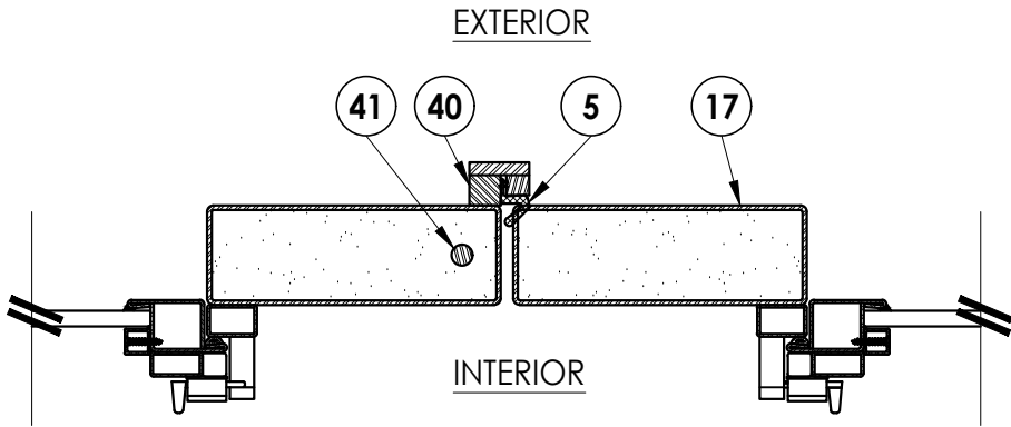
2 HORIZONTAL CROSS SECTION 3 Inswing Shown (Outswing Similar)
