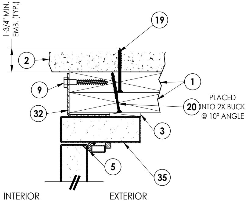
3 VERTICAL CROSS SECTION 3 Inswing Shown (Outswing Similar)
