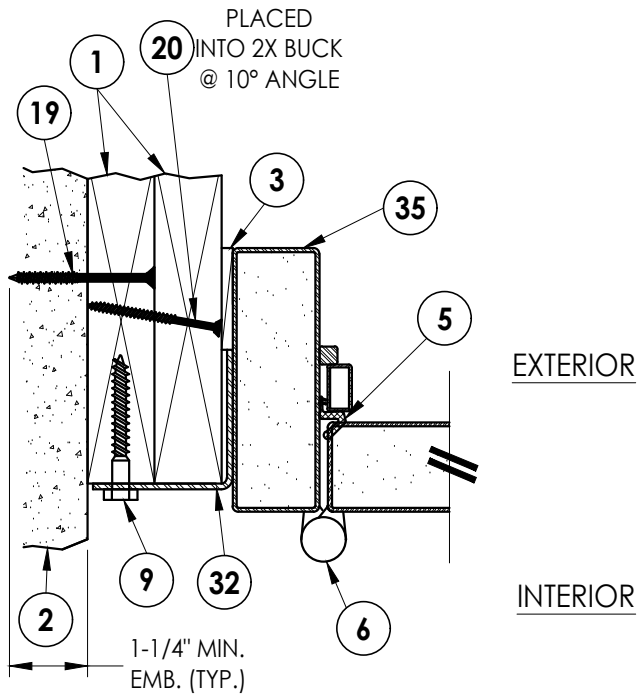
1 HORIZONTAL CROSS SECTION 3 Inswing Shown (Outswing Similar)
