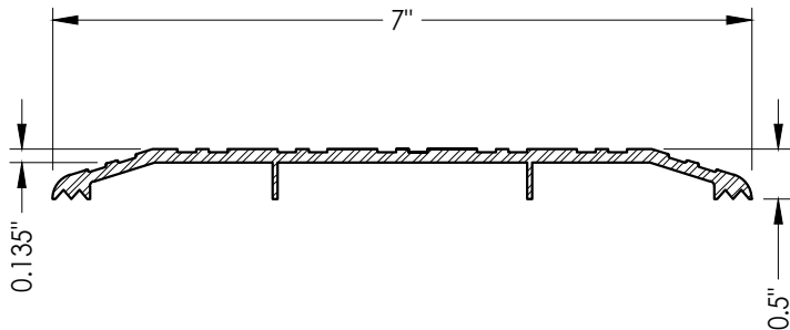
30 ADA THRESHOLD
