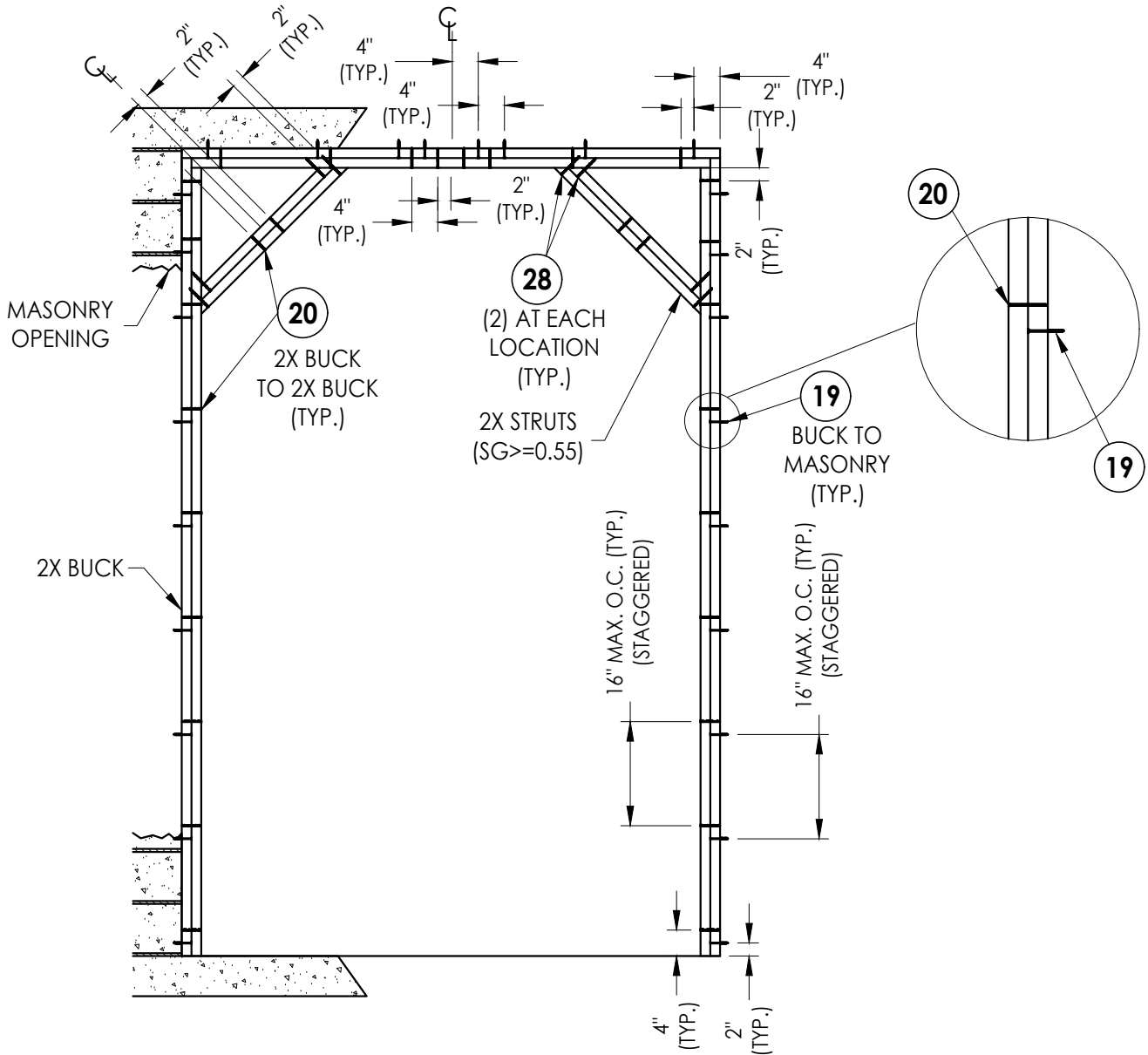
BUCK ANCHORING (Max. design pressure \pm 65 psf)
