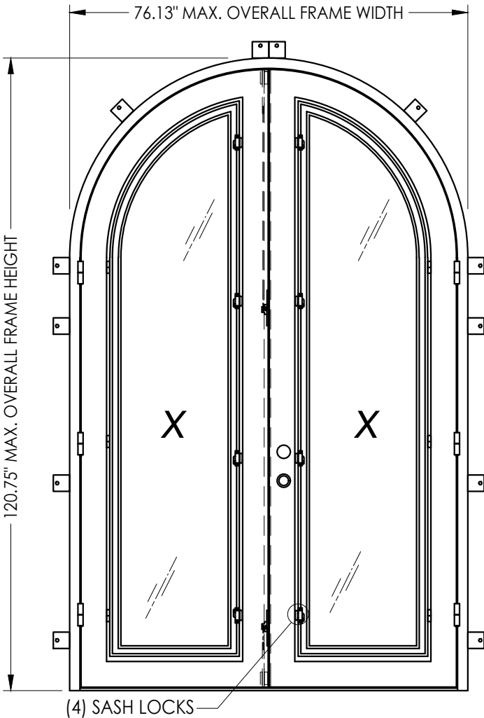
GLAZED DOOR WITH 4 SASH LOCKS
