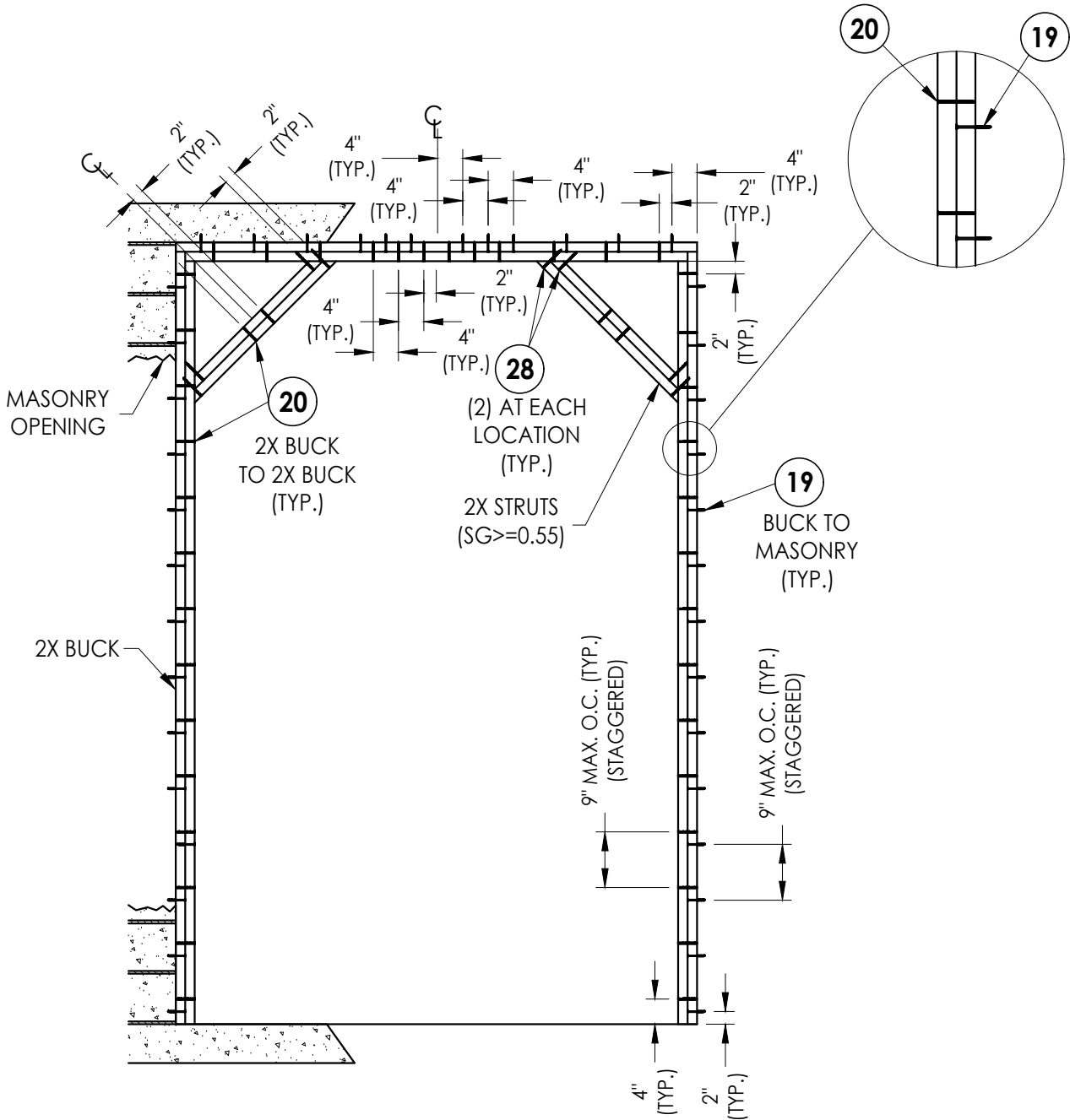
BUCK ANCHORING (Max. design pressure \pm 100 psf)
