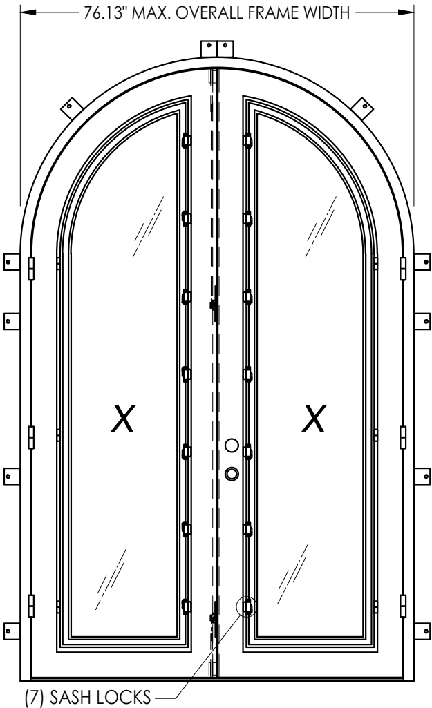
GLAZED DOOR WITH 7 SASH LOCKS
